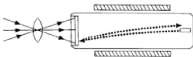
The Vidicon
