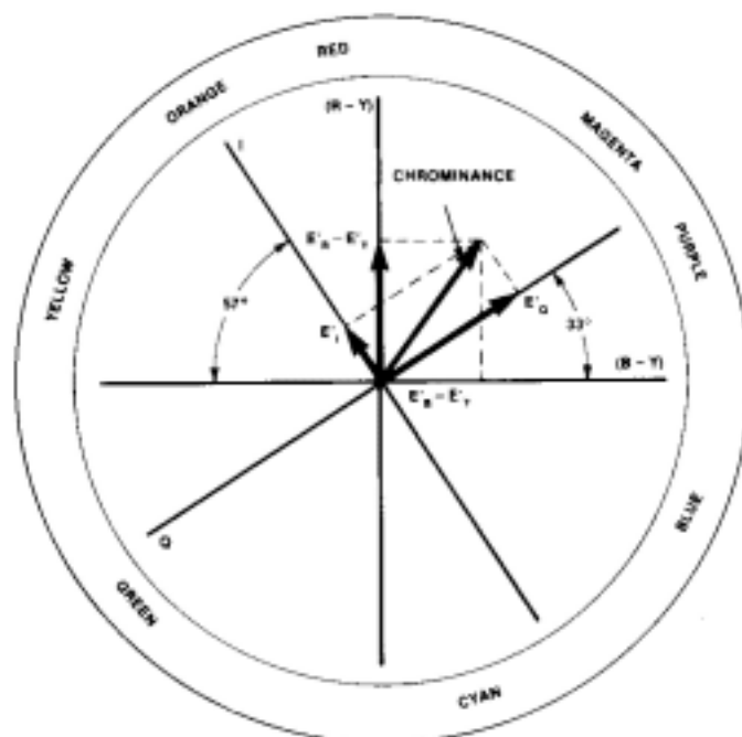
Lumiance, Chrominance, Saturation and Hue
