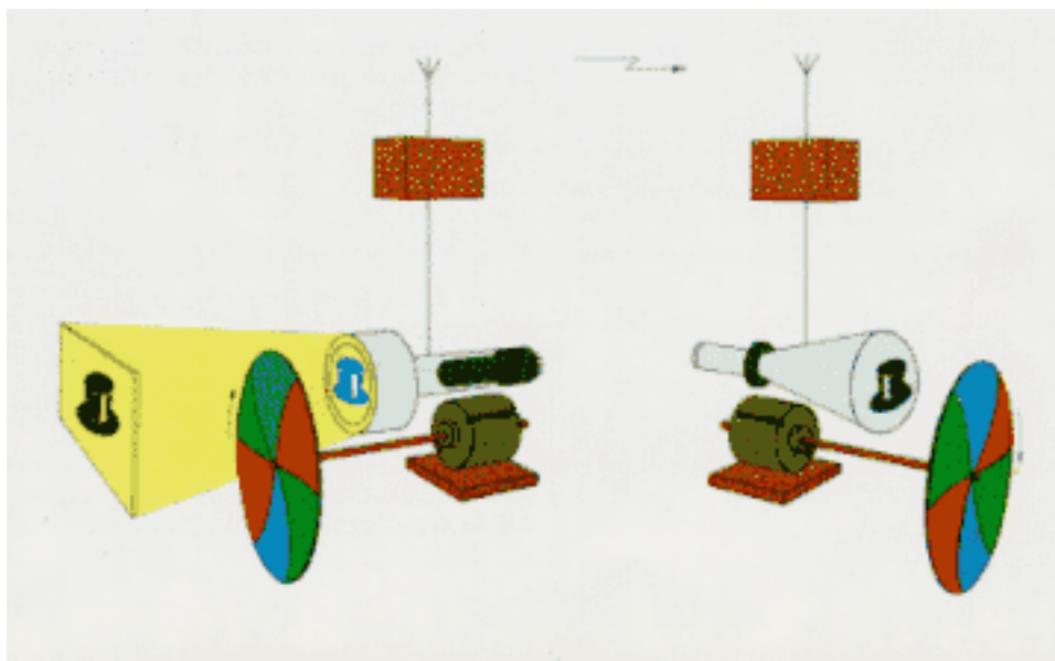
Goldmark's sequential three-filter system
