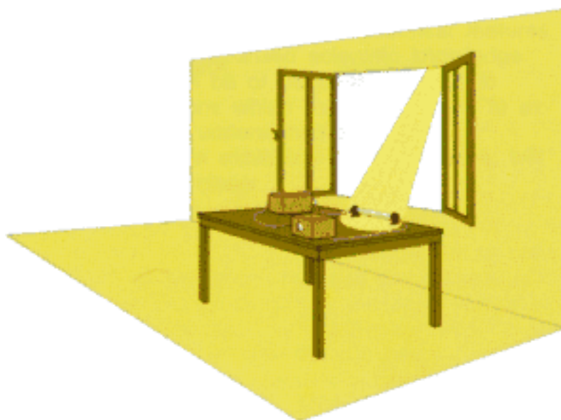
The photoelectric effect
