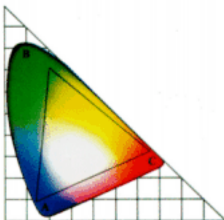
Television colour triangle
