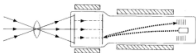
Image Orthicon
