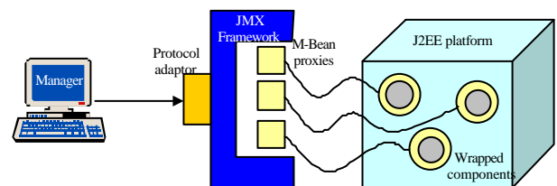
Figure 7. Solution being developed for MKBEEM prototype
