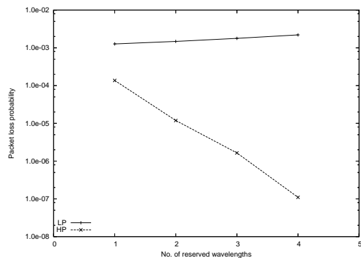
Fig. 7. QoS differentiation between HP and LP traffic in a 5 node OPS network as a function of the number of wavelengths reserved for HP traffic.
