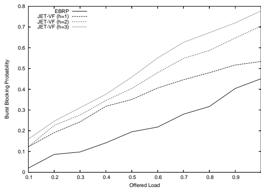
Fig. 6. Burst blocking probability of EBRP versus Just-Enough-Time with void filling (JET-VF) for bursts traversing through h=1, 2 or 3 nodes.
