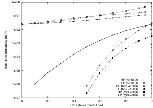
Fig. 4. Burst Loss Probabilities for HP and LP class as a function of HP traffic load.
