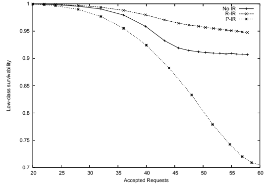
Fig. 1. Low-class survivability in a multi-service wavelength-routed optical network.
