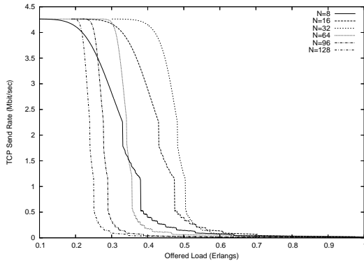
Fig. 5. TCP send rate as a function of the offered load per wavelength, varying the number of wavelengths per link as a parameter, wc = 64
