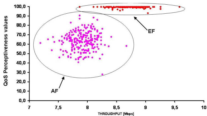
Fig. 8. QoS perceptiveness values vs throughput for EF and AF CoS, in case of a traffic load equal to 900 Mb/s in case of a tennis match video 30 second long.
