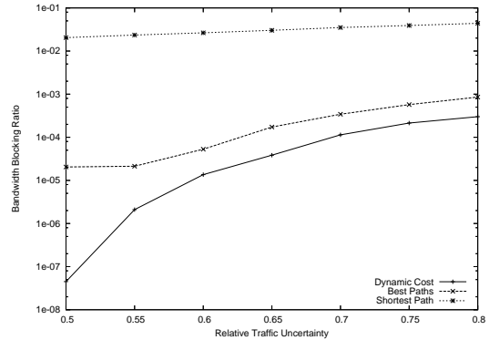
Fig. 2. Bandwidth Blocking Ratio as a function of the Relative Traffic Uncertainty for three routing strategies applied on a 10-node topology
