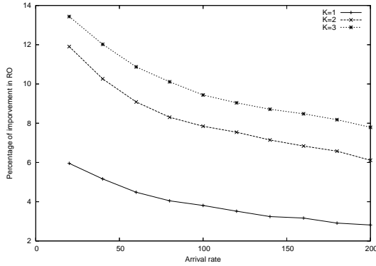
Fig. 3. RO as a function of calls arrival rate.
