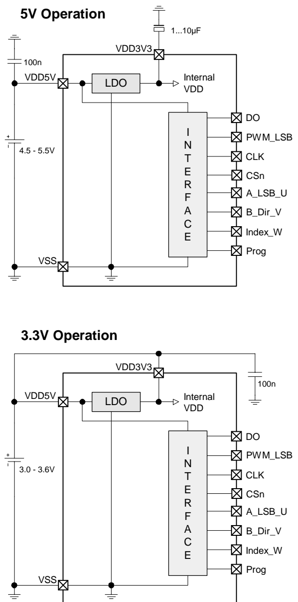
Figure 18: Connections for 5V / 3.3V supply voltages
