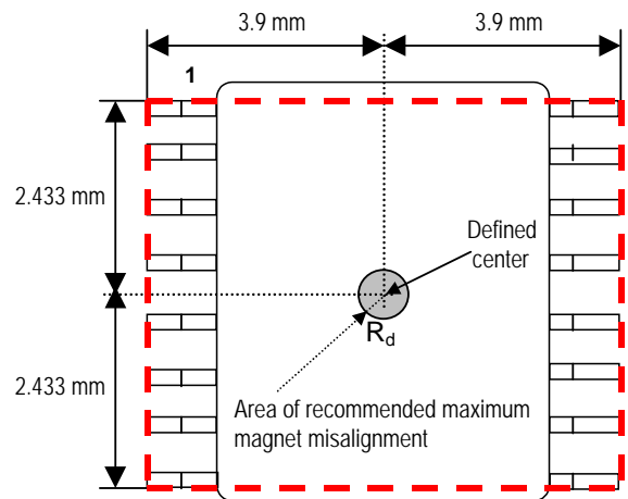
Figure 20: Defined IC center and magnet displacement radius
