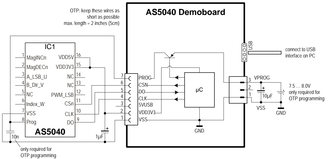
Figure 15: OTP programming connection of AS5040 (shown with AS5040 demoboard)
