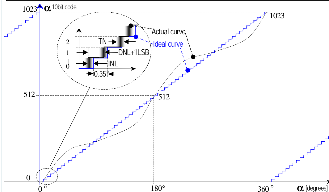
Figure 25: Integral and differential non-linearity example (exaggerated curve)
