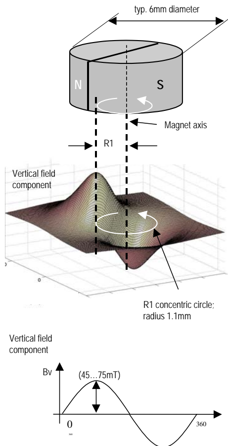
Figure 19: Typical magnet and magnetic field distribution
