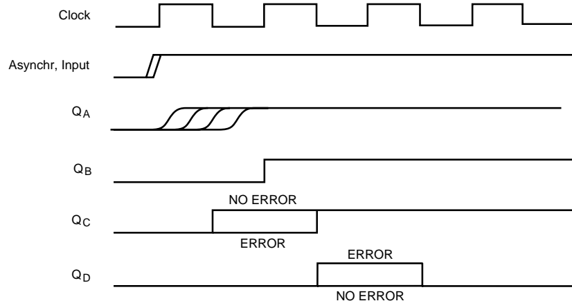
Figure 1: Test Circuit and Timing Diagram
