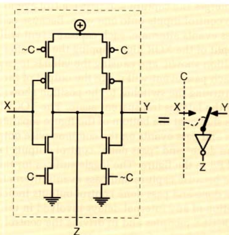
FIGURE 11. Circuit for the Switch Symbol
