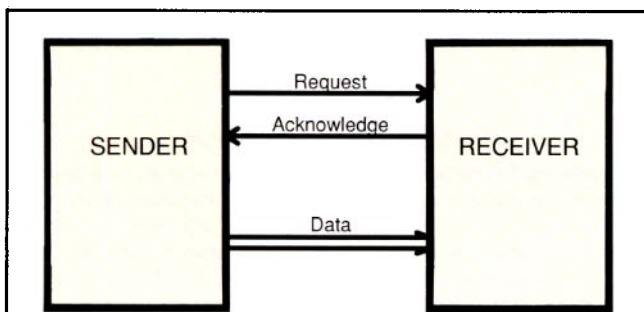
FIGURE 3. A Bundled Data Interface
