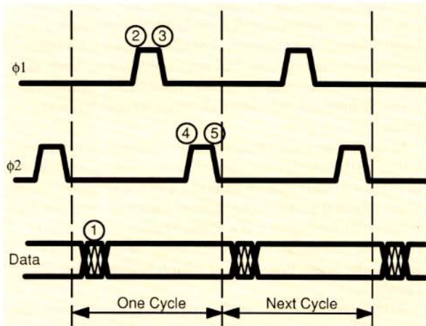
FIGURE 5. Nonoverlapping Clocks
