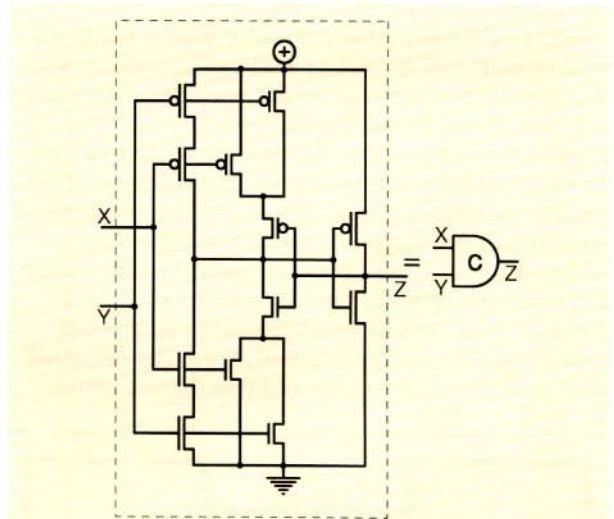
FIGURE 7. A Static Muller C-Element
