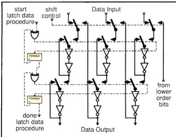
FIGURE 22. Data Path for Sequential Normalizer
