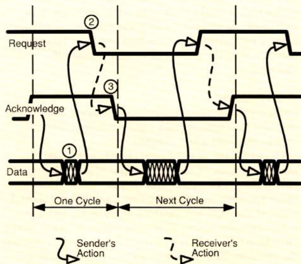
FIGURE 4. The Two-phase Bundled Data Convention
