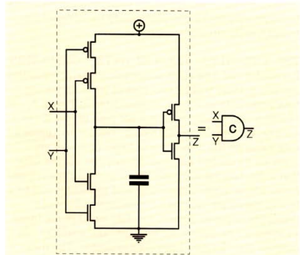
FIGURE 6. A Dynamic Muller C-Element
