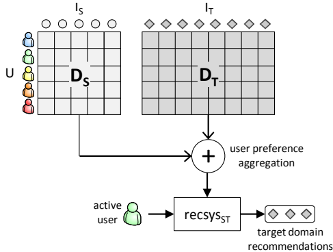
Fig. 5 Merging user preferences. Data sources from different domains are merged, and a traditional single-domain recommender system is used on the merged data.
