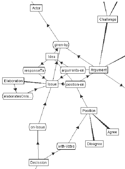
Figure 2. Main concepts of the argumentation ontology
