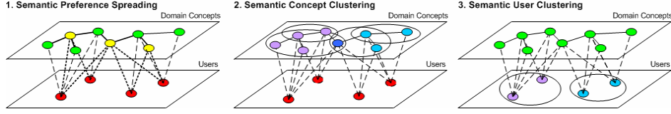
Fig. 1. Overall sequence of our proposed approach, comprising three steps: 1) semantic user preferences are spread, extending the initial sets of individual interests, 2) semantic domain concepts are clustered into concept groups, based on the vector space of user preferences, and 3) users are clustered in order to identify the closest class to each user
